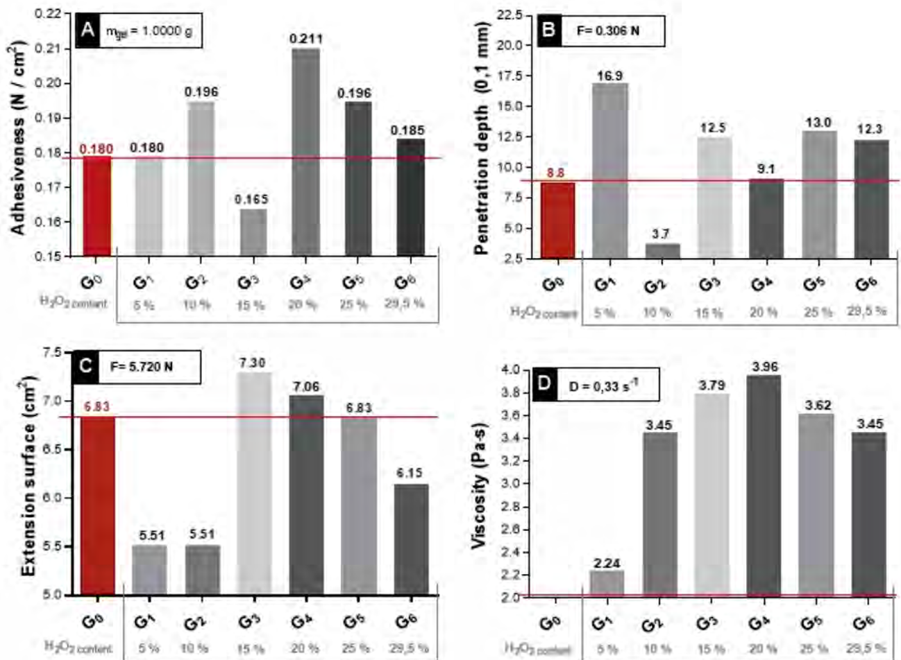
FIGURE 1. Rheological parameters that characterize the studied gels: adhesiveness (A), consistency (B), extensibility (C), viscosity (D)
