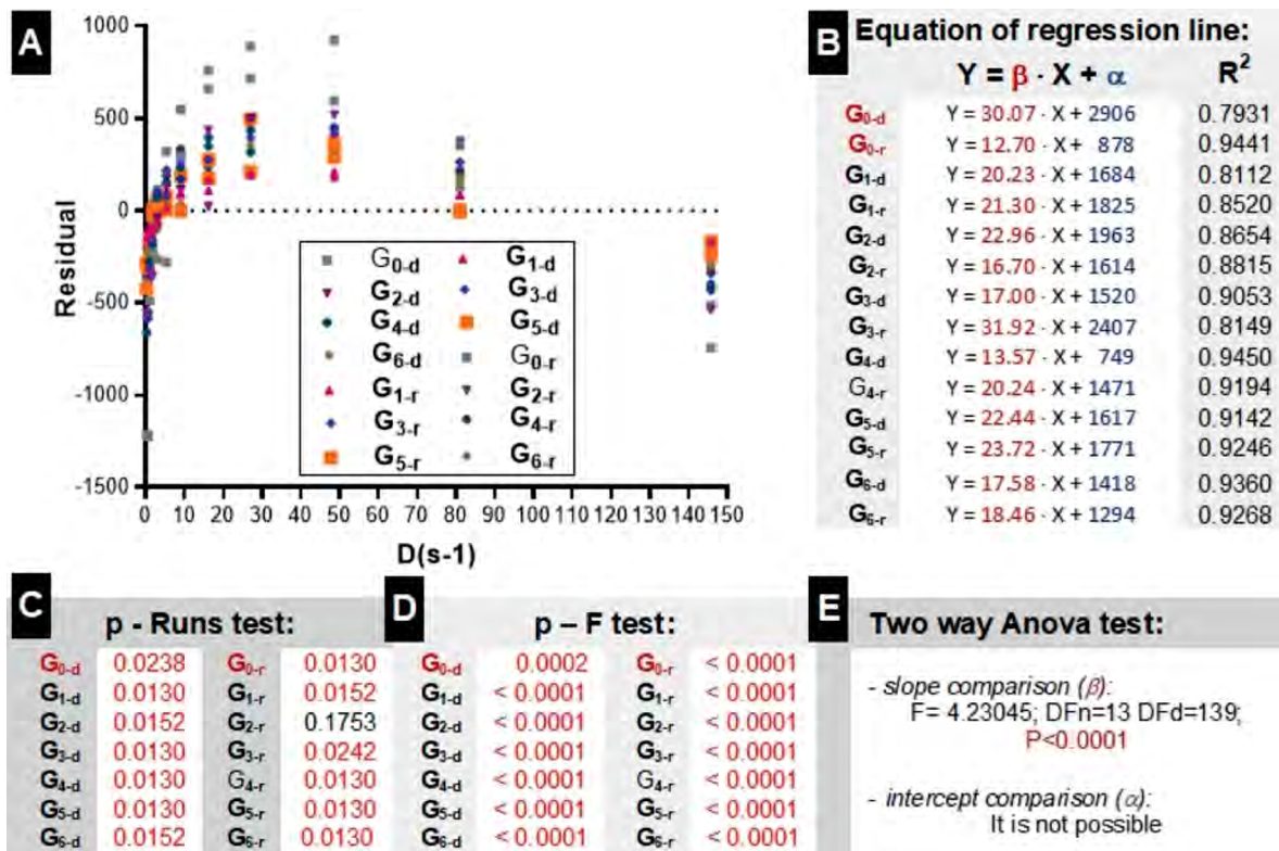
FIGURE 3. Analysis of flow curves by linear regression: residuals (A), equation of regression lines (B), deviation from linearity (C), deviation from zero (D), results of the variance test (E)
