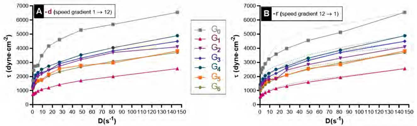
FIGURE 2. Flow curves: destructuring stage - d (A), restructuring stage - r (B)
